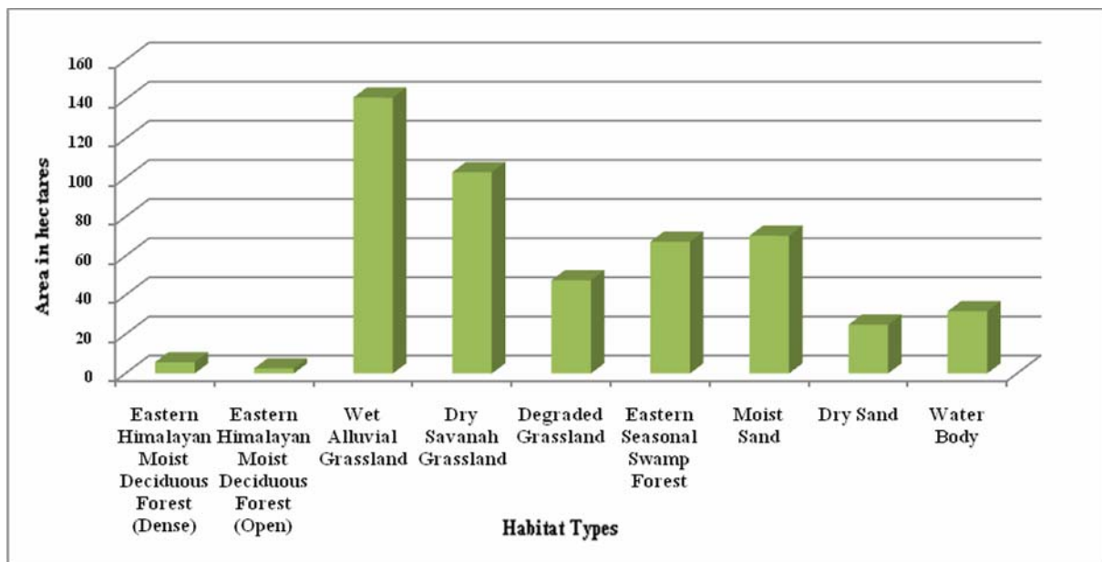
Fig. V g) Habitat pattern of Jhawani Block
