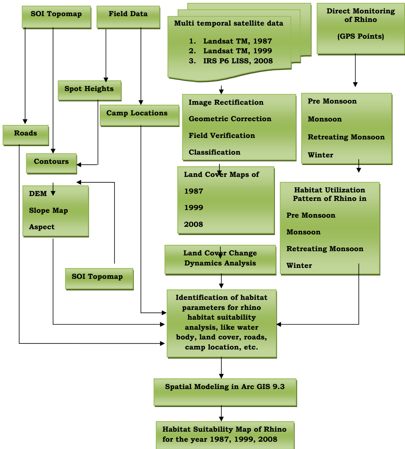
Fig. II. e) - General methodology of the study
