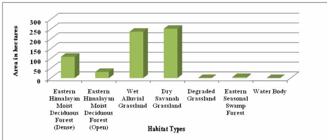
Fig. V h) Habitat pattern of Magurmari Block
