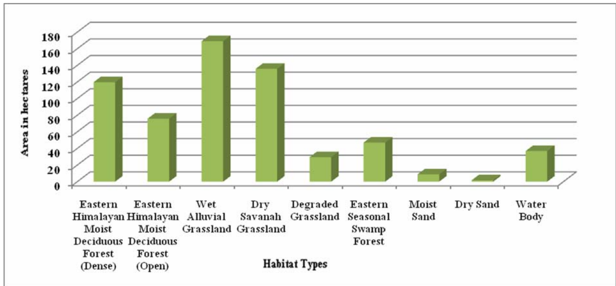
Fig. V j) Habitat pattern of Oogli Block
