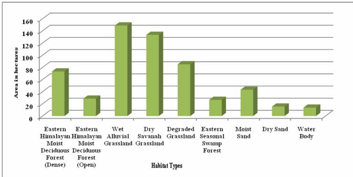
Fig. V q) Habitat pattern of Solmari Block
