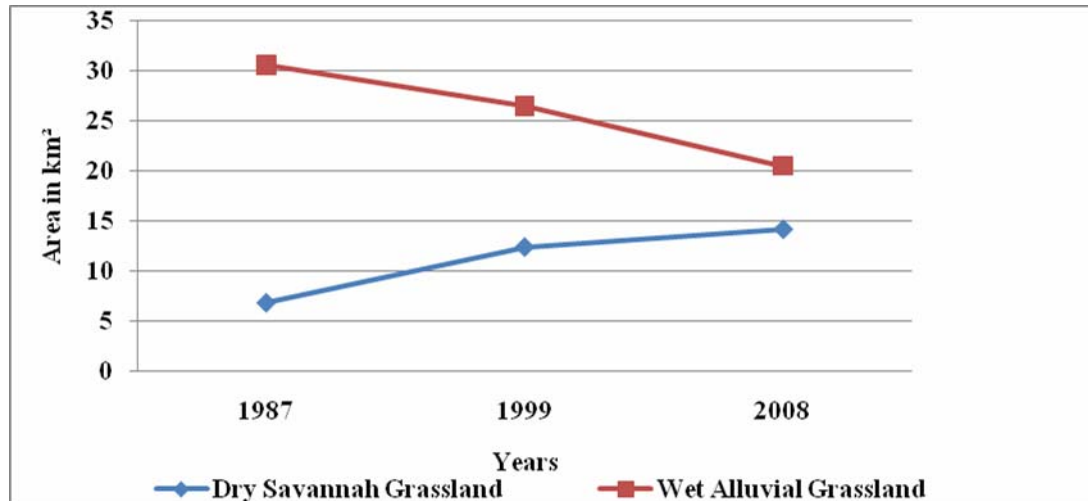
Fig. III d) Changes in Wet Alluvial and Dry Savannah Grassland in Orang NP from 1987 to 2008
