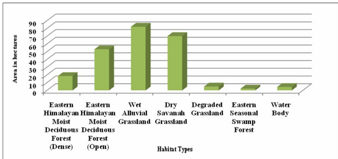
Fig. V b) Habitat pattern of Baghmari Block
