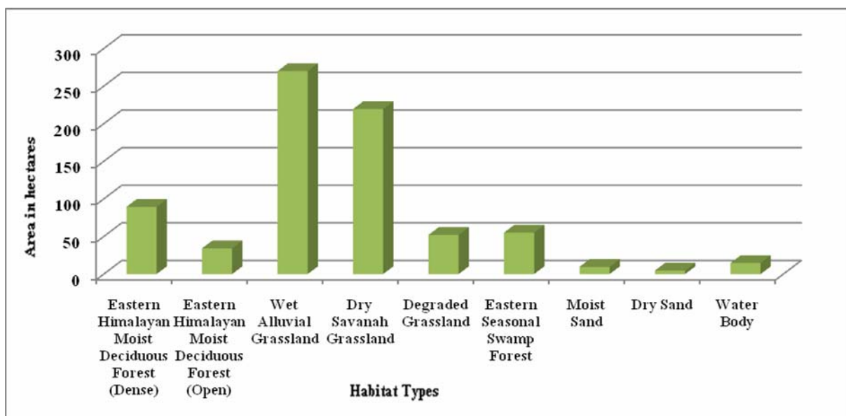
Fig. V n) Habitat pattern of Ramdas Block
