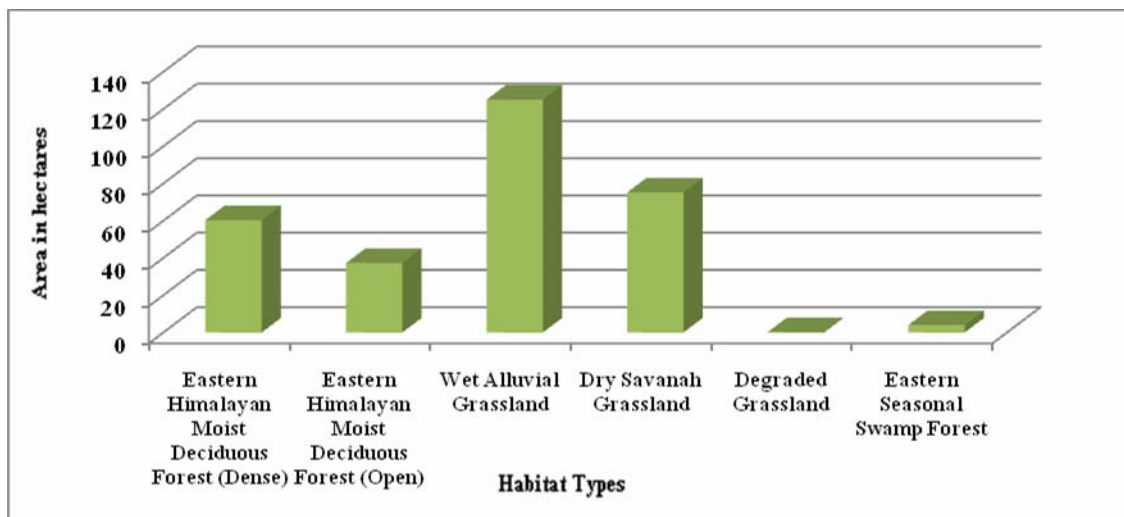
Fig. V i) Habitat pattern of Moalamari Block
