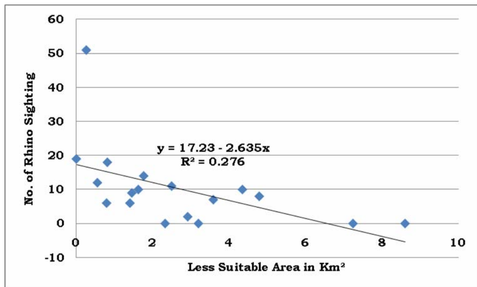
Fig. VI q) Relationship between less suitable habitat and number of rhino sighting
