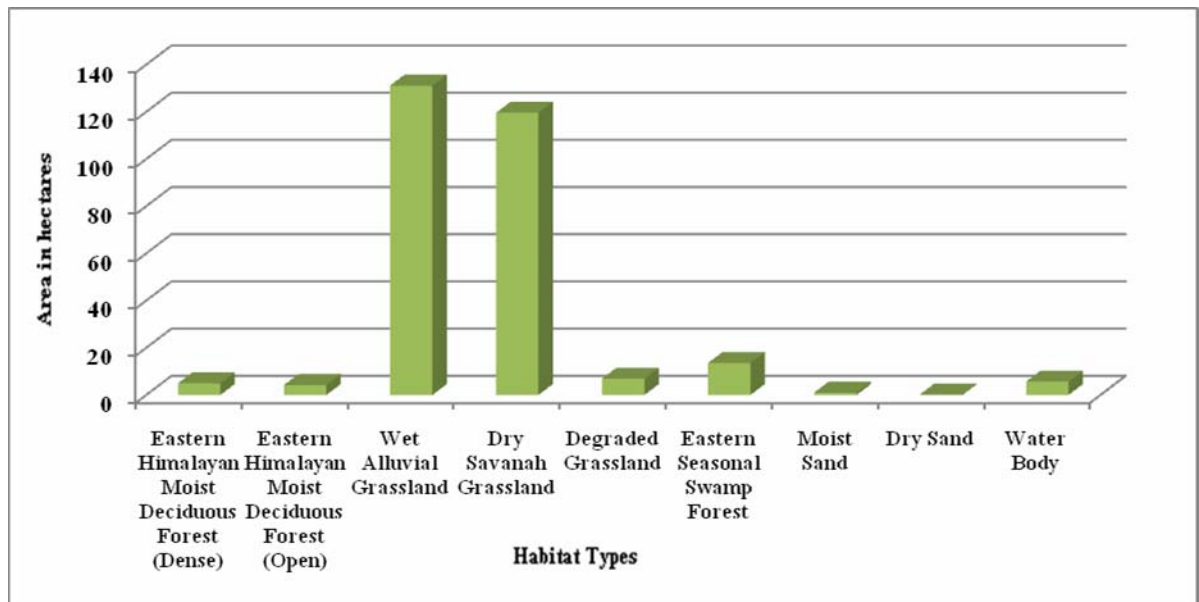
Fig. V e) Habitat pattern of Chiala Block
