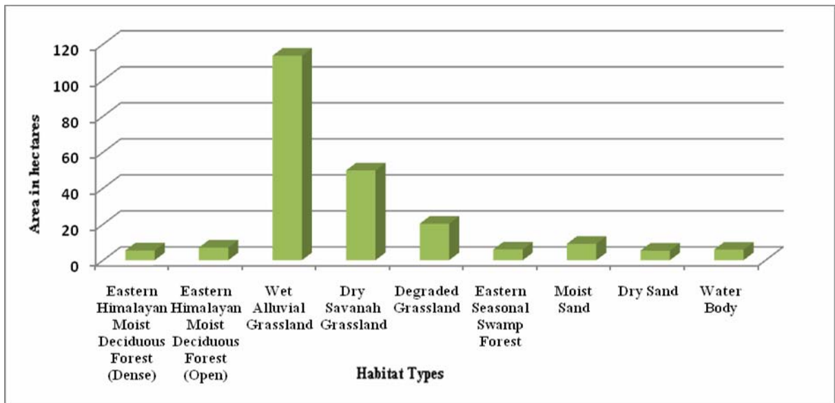
Fig. V k) Habitat pattern of Pabhomari Block
