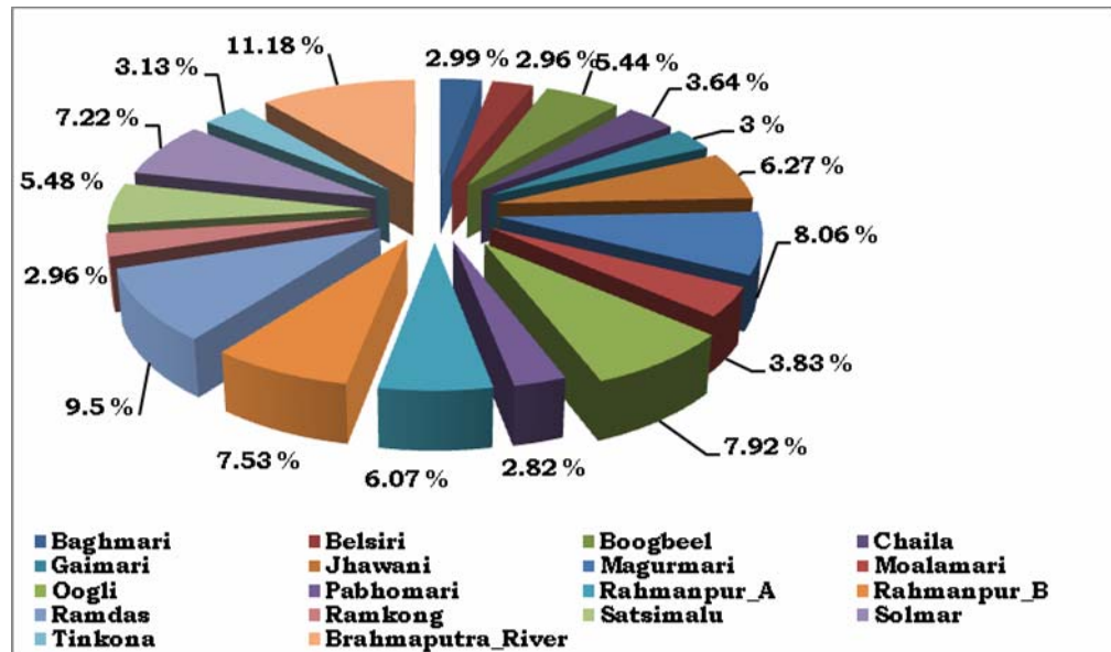
Fig. V a) Percentage area covers by each block of RG Orang NP
