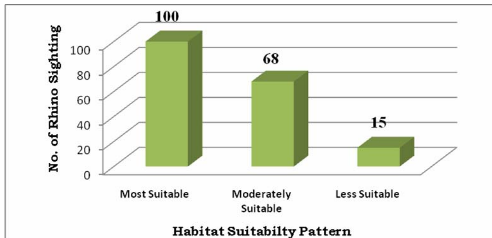
Fig. VI n) Distribution of rhino in different habitat suitability categories.
