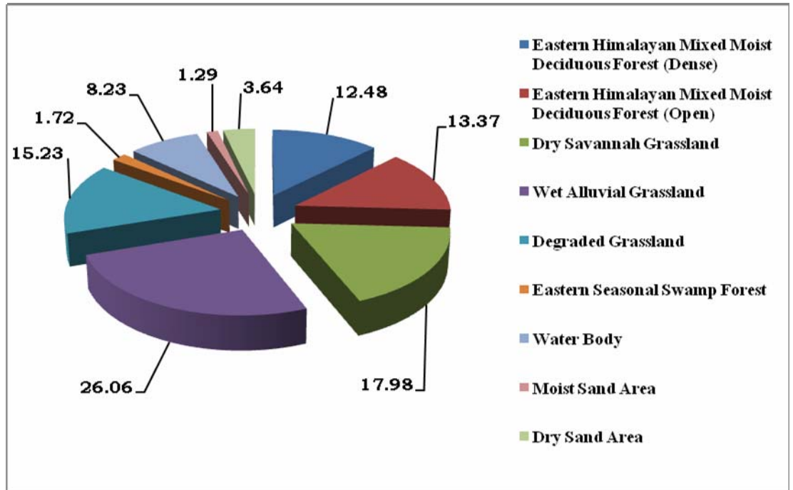
Fig. III a) Land cover pattern of RG Orang NP in 2008 (in %)
