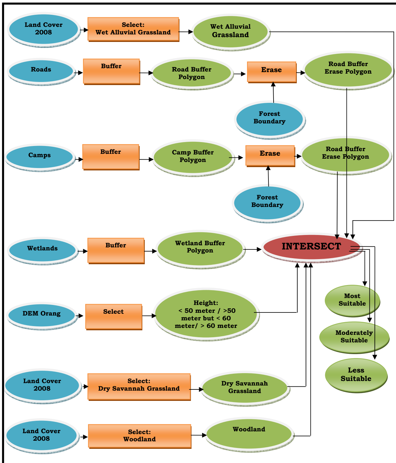
Fig. VI f) Rhino Habitat Suitability Model
