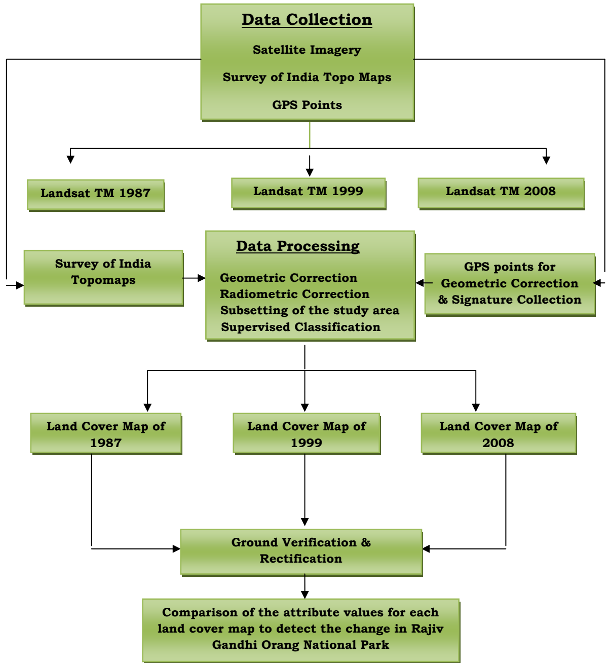
Fig. II. c. Flow Chart for land cover change dynamics analysis
