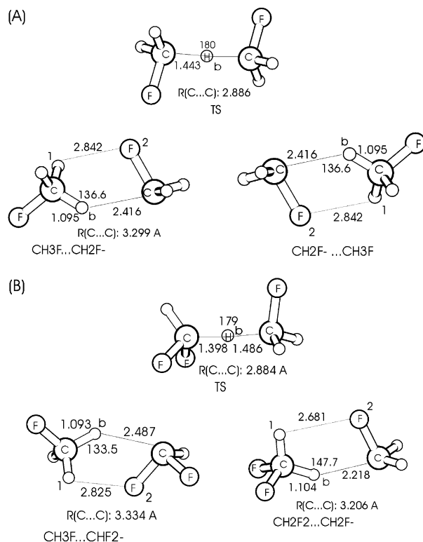
Figure 1. B3LYP/6-311++G(d,p) optimized geometries of CH _3\text{F}\cdots\text{CH}_2\text{F}^- CH _3\text{F}\cdots\text{CHF}_2^- (stable complex) and CH _2\text{F}\cdots\text{CH}_2\text{F}^- (metastable complex). The geometry of the corresponding transition states (TS) is also shown.
