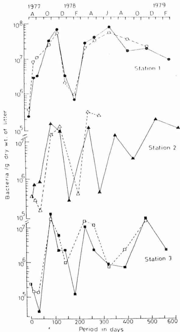
Fig. 2. Bacterial population associated with decomposing plant litter at various collections during the study period. Solid lines: pine needle; broken lines: teak leaf.
