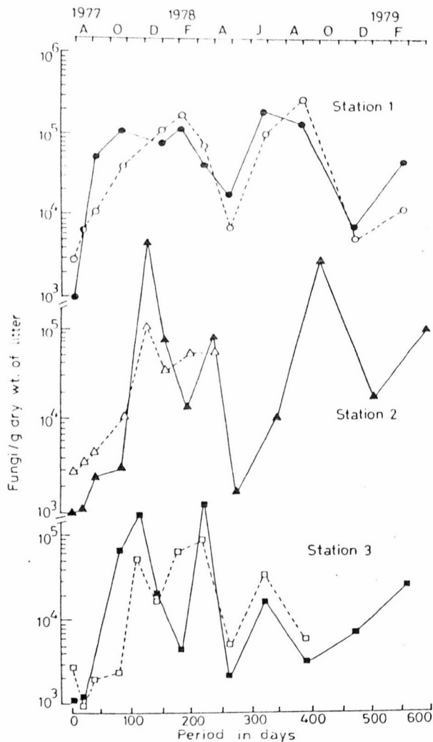
Fig. 3. Fungal population associated with decomposing plant litters at various collections during the study period. Solid lines: pine needle; broken lines: teak leaf.
