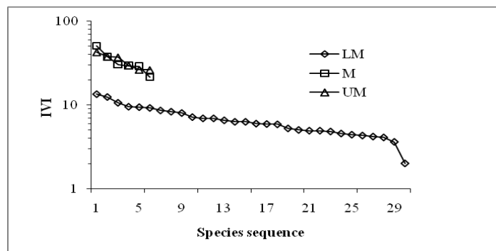
Figure 4.5. Dominance-diversity curve for shrub species in Lower montane (LM), Montane (M) and Upper montane (UM) forests in KBR.
