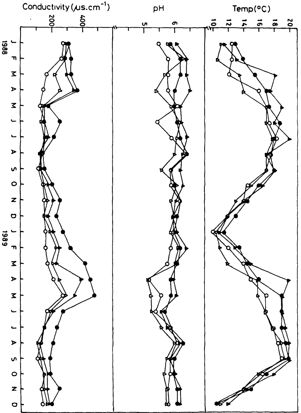
Fig. 3.1 Monthly variations in water temperature, pH and conductivity at four selected stations: 1 ( \Delta ), 2 ( \blacktriangle ), 3 ( \circ ) and 4 ( \bullet ).
