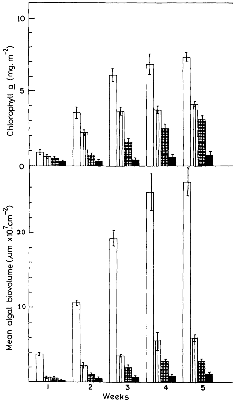
Fig. 6.2 Weekly variations in chlorophyll a concentration (mg m -2 ) and mean algal biovolume (μm 3 x 10 7 cm -2 ) under four light conditions; □ Exposed; ▨ Partially-shaded; ▩ Partially-exposed; and ■ shaded.
