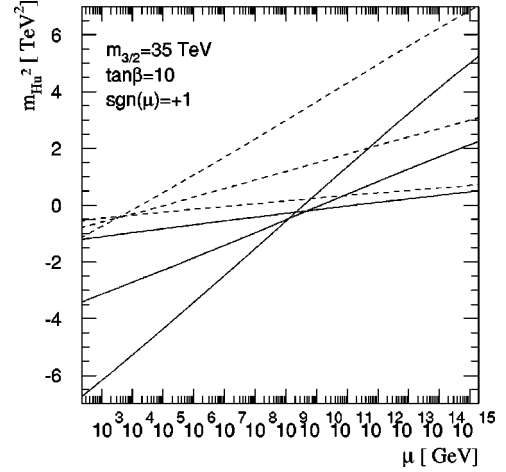
FIG. 3. Focus points for the minimal (dashed line) and gaugino assisted (solid line) AMSB models.
