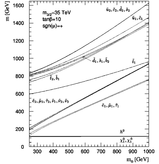
FIG. 5. The spectrum of the gaugino assisted AMSB model.
