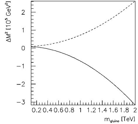
FIG. 2. The average mass difference \Delta M^2 \equiv 2\sum M_{\tilde{\chi}_i^\pm}^2 - \sum M_{\tilde{\chi}_i^0}^2 in the AMSB models (solid line), and in the minimal SUGRA (dashed line) as a function of the gluino mass m_{\tilde{g}} .
