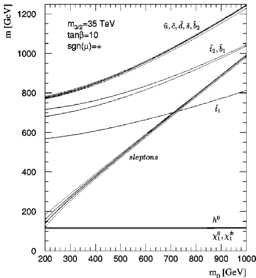
FIG. 4. The spectrum of the minimal AMSB model.
