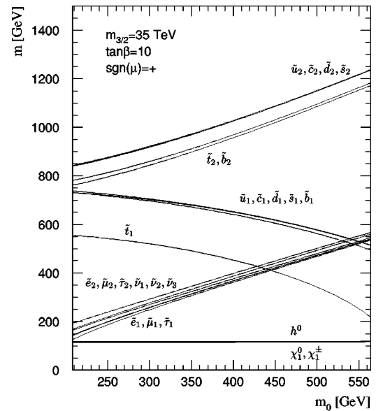
FIG. 6. The spectrum of the U(1) model.
