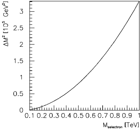
FIG. 1. The difference \Delta M^2 \equiv M_{u_R}^2 - M_{d_R}^2 as a function of the right-handed selectron mass M_{\tilde{e}_R} . We have plotted the curve for \tan \beta = 10 , but the curves for \tan \beta > 3 are all almost identical.
