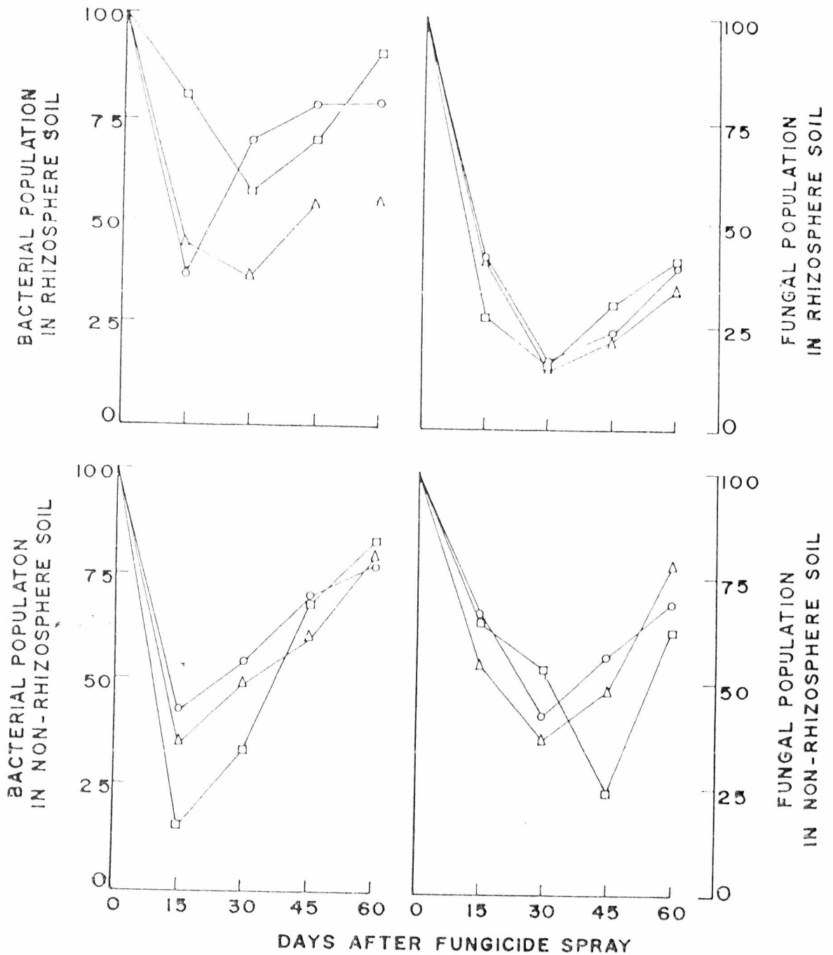
Figure 1 Bacterial and fungal population in non-rhizospheric and rhizospheric soil sprayed with fungicides
