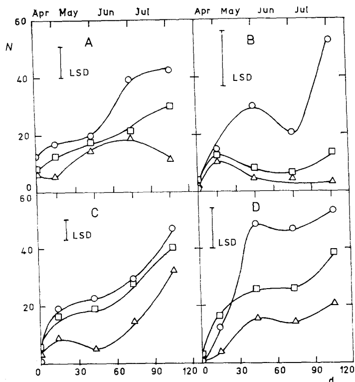
FIG. 2. Colonization of bacterial population in the different types of fuel-burned soil (year 1980); N — number of bacteria per g dry soil \times 10^{-5} ; for further symbols see Fig. 1.
