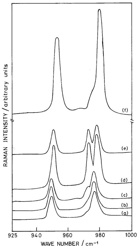
Figure 1. The observed Raman spectra of TB10A in the region 925\text{--}1000 \text{ cm}^{-1} at different temperatures during a cooling cycle: (a) 229 K; (b) 135 K; (c) 93 K; (d) 47 K; (e) 20 K; (f) room temperature spectrum recorded separately.
