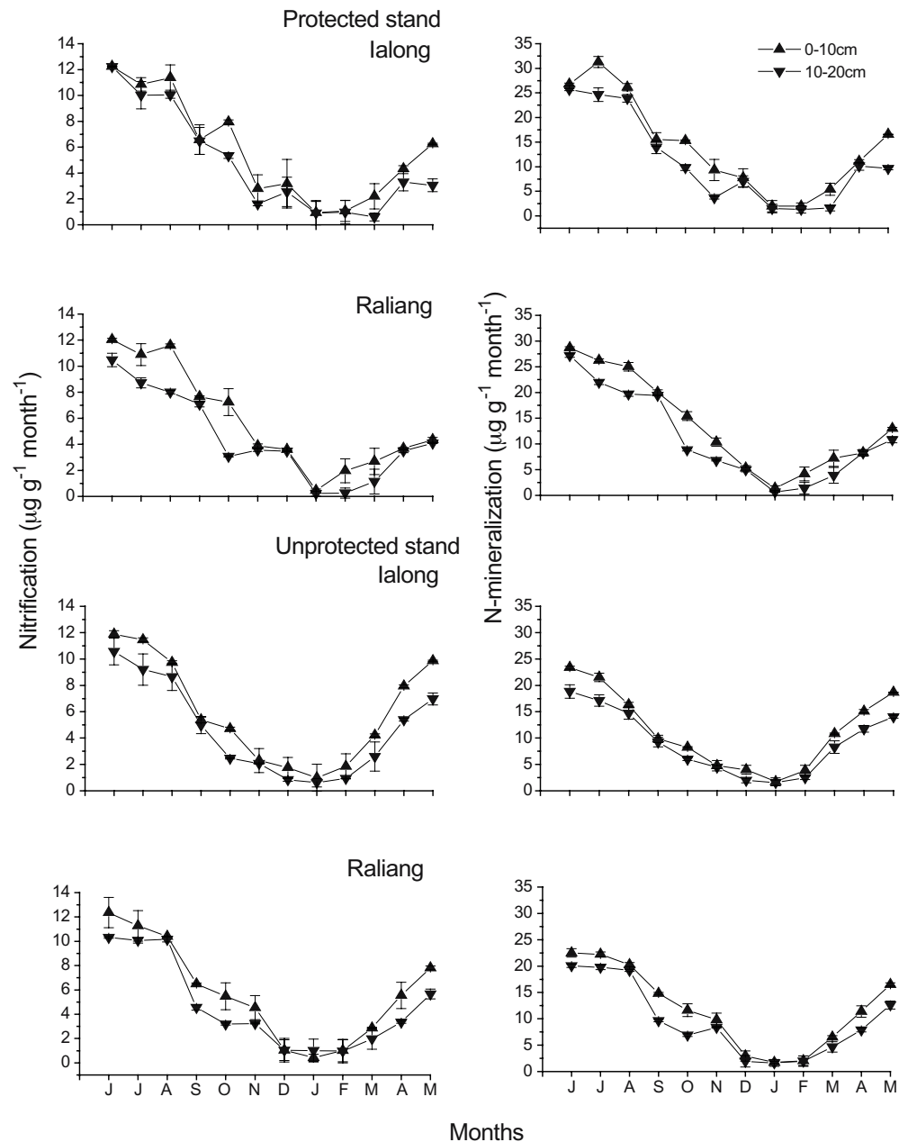
Fig. 3 Monthly variation of nitrification and net N mineralization rate in protected and unprotected stands of subtropical forest at Ialong and Raliang
