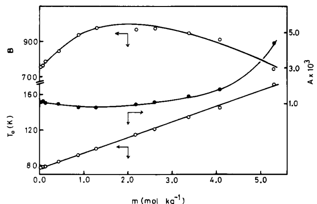
Figure 2. Plots of A , B , and T 0 parameters versus m for the NiCl 2 + CH 3 OH system.
