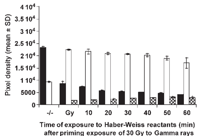
Figure 7. Bar diagrams showing the net intensity of the OC, L and CC bands of pMTa4 resolved on agarose gel (not shown) after exposure to a priming dose of 30 Gy of \gamma -rays followed by Haber–Weiss oxidants from 10 to 60 min. The closed, open and crossed bars represent the CC (native), OC (SSB) and L (DSB) forms, respectively. The first set of bars marked -/- is for sham-exposed control, the second set of bars marked Gy is for pMTa4 exposed only to \gamma -rays (30 Gy) while the remaining sets of bars are for samples exposed to \gamma -rays followed by increasing periods of Haber–Weiss oxidants.
