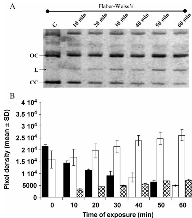
Figure 2. DNA strand breaks induced by Haber-Weiss reactants. Panel A shows the electrophoreogram of plasmid pMTa4 unexposed (C) or exposed to Haber-Weiss oxidant from 10 to 60 min. The bands marked CC, OC and L represent the undamaged native, SSB induced and DSB induced forms of the plasmid, respectively. Panel B shows the net intensities of the bands (mean \pm SD) in form of a bar diagram. The closed, open and crossed bars represent the CC (native), OC (SSB), L (DSB) forms, respectively.
