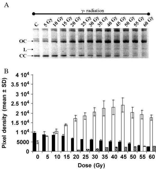
Figure 3. DNA strand breaks induced by \gamma -rays. Panel A shows the electrophoreogram of plasmid pMTa4 unexposed (C) or exposed to different doses of \gamma -rays (5–60 Gy). The bands marked CC, OC and L represent the undamaged native, SSB induced and DSB induced forms of the plasmid, respectively. Panel B shows the net intensities of the bands (mean \pm SD) in form of a bar diagram. The closed, open and crossed bars represent the CC (native), OC (SSB), L (DSB) forms, respectively.
