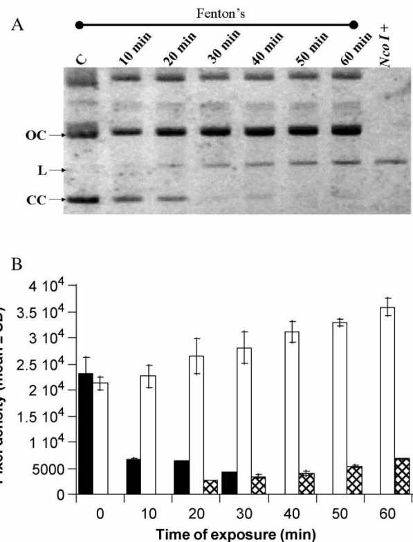
Figure 1. DNA strand breaks induced by Fenton reactants. Panel A shows the electrophoreogram of plasmid pMTa4 unexposed (C) or exposed to Fenton oxidant from 10 to 60 min. The bands marked CC, OC and L represent the undamaged native, SSB induced and DSB induced forms of the plasmid, respectively. The last lane marked Nco I + was loaded with pMTa4 linearized with restriction enzyme Nco I . Panel B shows the net intensities of the bands (mean \pm SD) in form of a bar diagram. The closed, open and crossed bars represent the CC (native), OC (SSB), L (DSB) forms, respectively.
