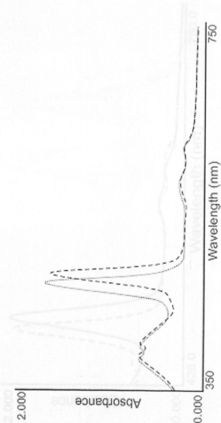
Figure 3.2.1.a. UV-Visible Absorption Spectrum of \text{Mn(III)[T(2-OMeP)P]OAc} in \text{CH}_2\text{Cl}_2 at room temperature (-----); on addition of 0.1 ml of Diethylamine (————).
