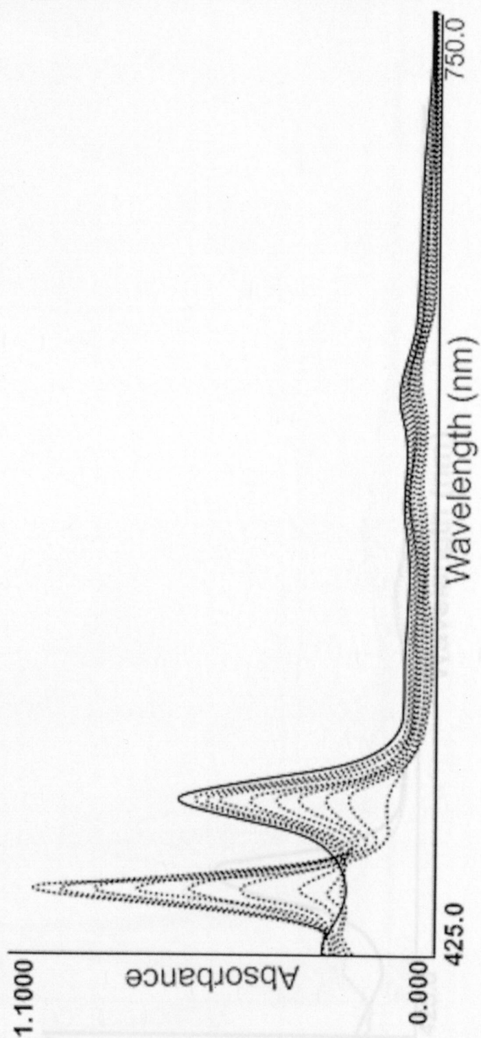
Figure 3.2.2.c. UV-Visible Overlay Spectra of \text{Mn(III)[T(4-OMeP)POAc]} in \text{CH}_2\text{Cl}_2 at room temperature (—); on addition of Triethylamine (---).
