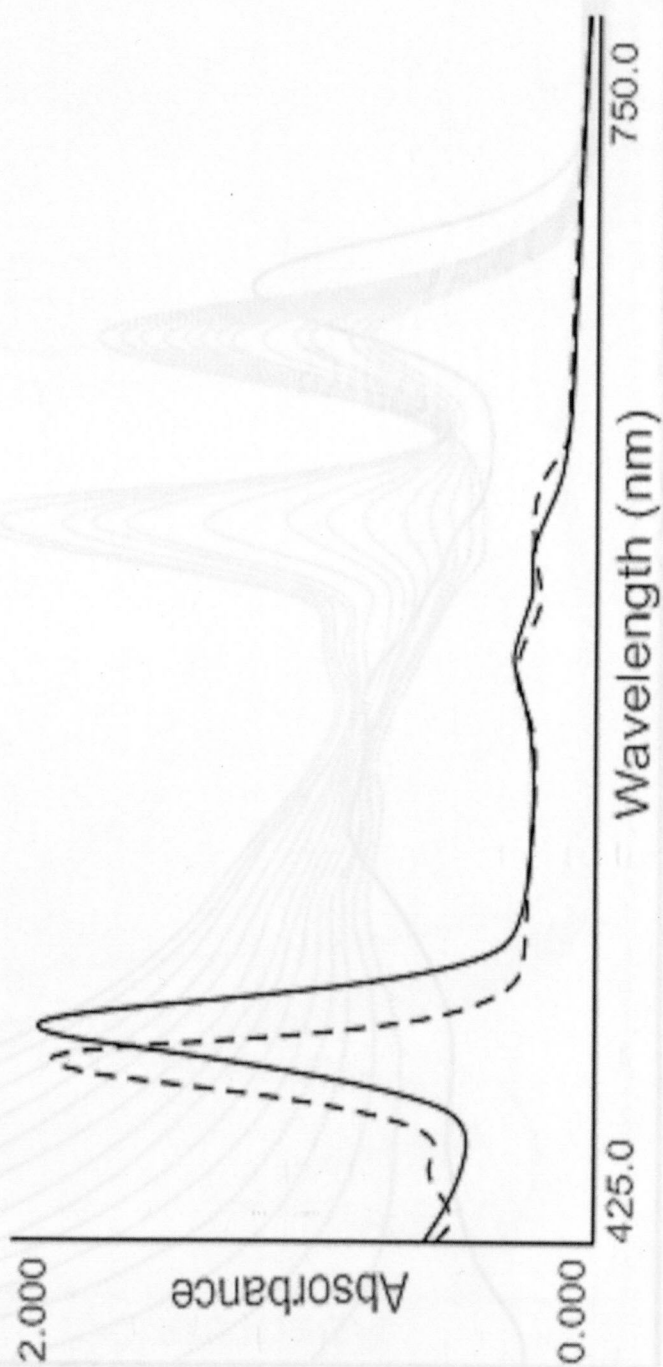
Figure 3.2.1.b. UV-Visible Absorption Spectrum of \text{Mn(III)[T(2-OMeP)P]OAc} in \text{CH}_2\text{Cl}_2 at room temperature (—); on addition of 0.3 ml of Diethylamine (---).
