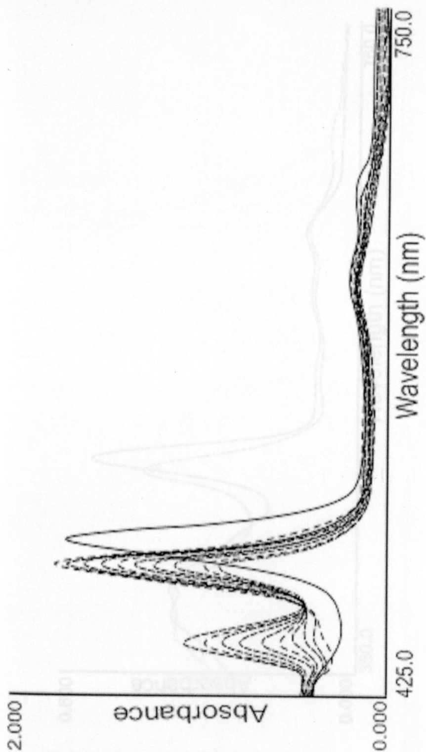
Figure 3.2.1.d. UV-Visible Overlay Spectra of \text{Mn(III)[T(2-OMeP)OAc]} in \text{CH}_2\text{Cl}_2 at room temperature (—); on addition of Triethylamine (---).
