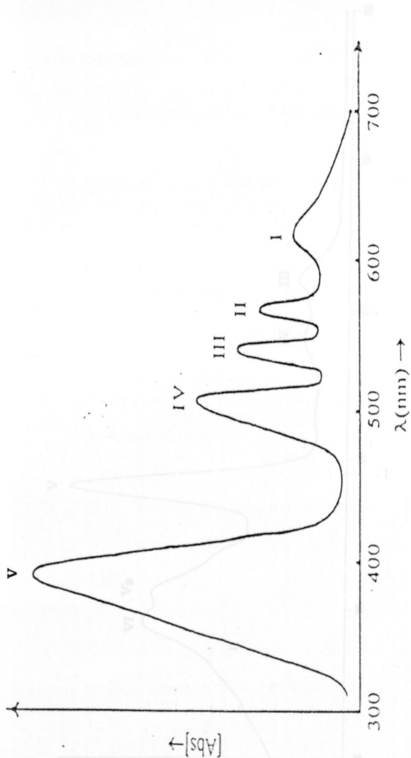
Figure: 1.4. UV-Visible Absorption Spectrum Of A Porphyrin.
