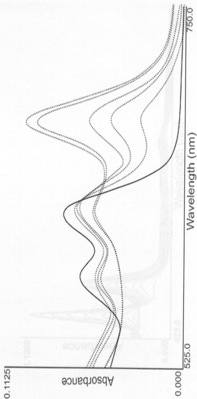
Figure 3.2.2.b. UV-Visible Absorption Spectrum of \text{Mn(III)[T(4-OMeP)OAc]} in \text{CH}_2\text{Cl}_2 at room temperature (—); on continuous addition of Diethylamine (— — —).
