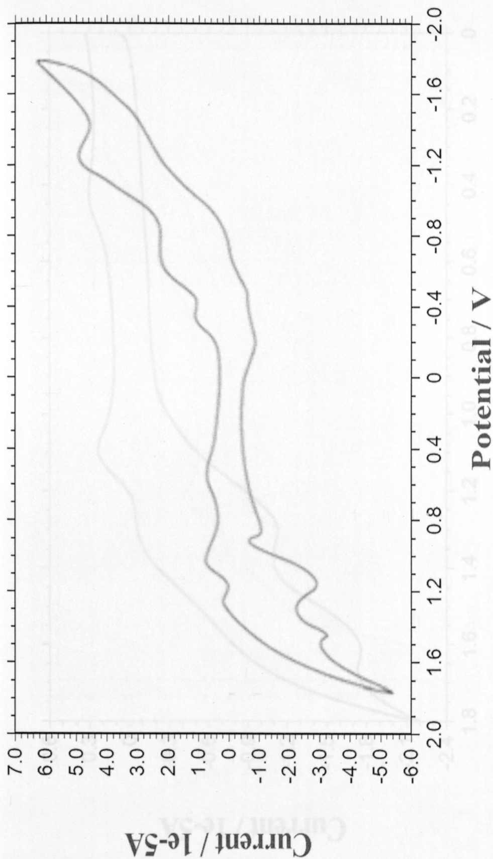
Figure: 4.2.1.a. Cyclic Voltammogram of \text{Mn(III)[T(2-OMeP)P]OAc} in \text{CH}_2\text{Cl}_2 containing 0.1M TBAP at Room Temperature.
