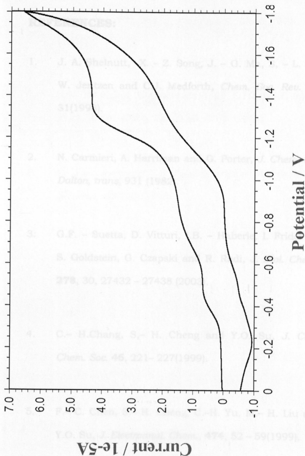
Figure: 4.2.3.b. Cyclic Voltammogram of Mn(III)[TNP]OAc in CH 2 Cl 2 containing 0.1M TBAP At Room Temperature
